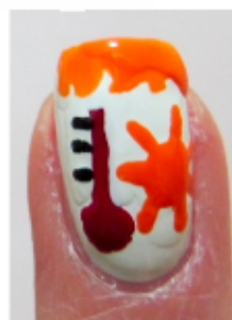
Global Warming
